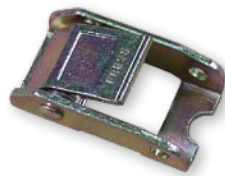
1" CAM BUCKLE 600 lb. working load cap. Model # 5K
